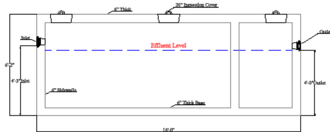
Elevation View
