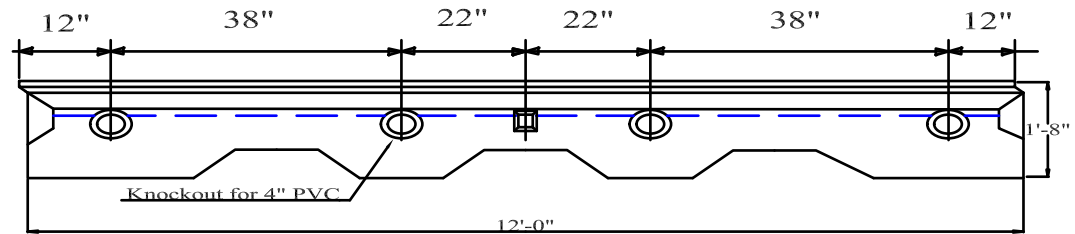
Plan View
