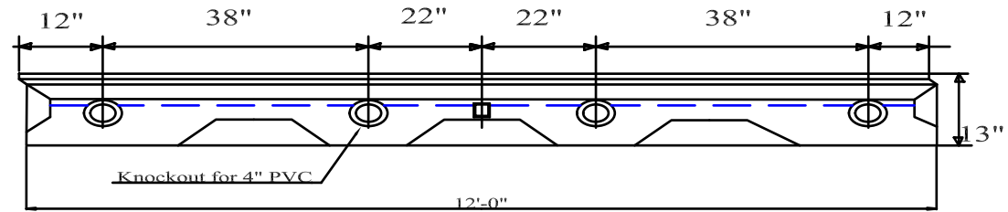
Elevation View
