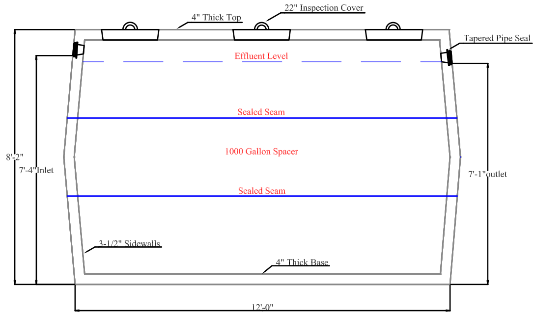
Elevation View
