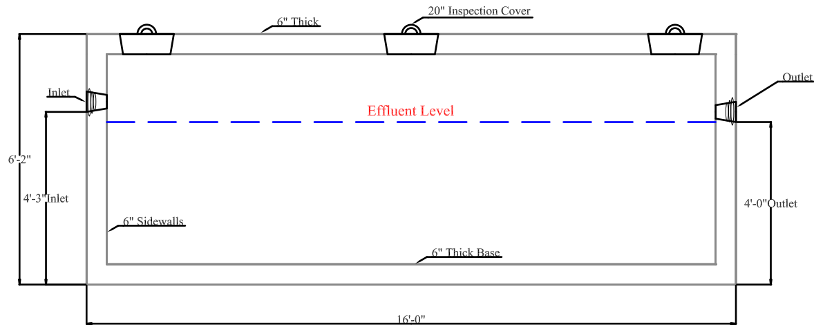
Elevation View
