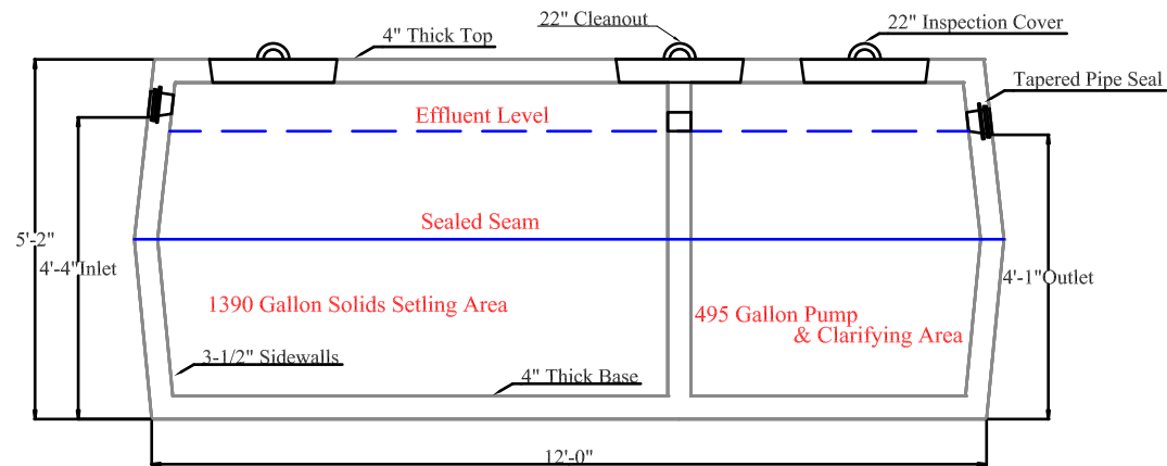
Elevation View
