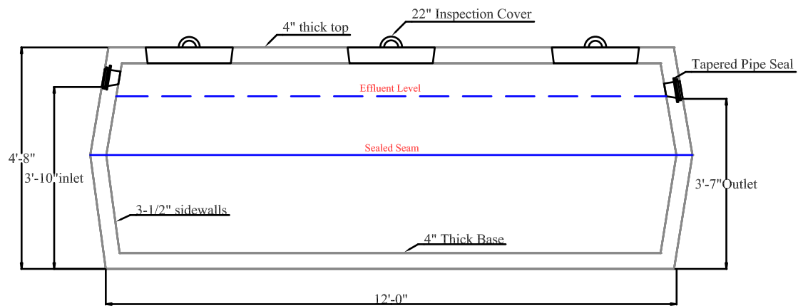
Elevation View
