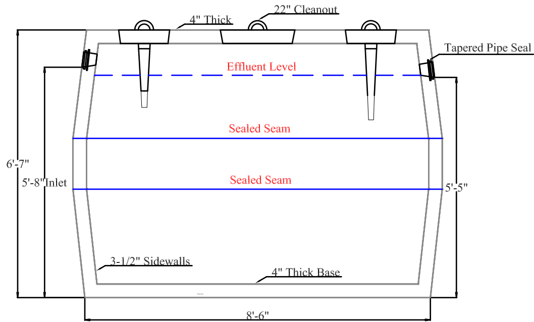
Elevation View
